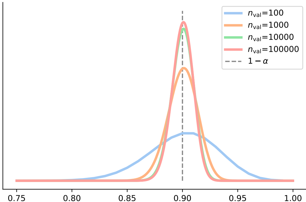
Distribution of coverage with n_{\text{val}} validation points ( n = 1000 )
